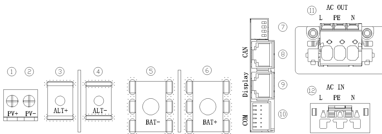
Figure 2-4 Terminal
