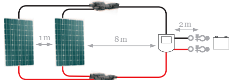
Connexion 2 panneaux = UNICONNECT 2.6
