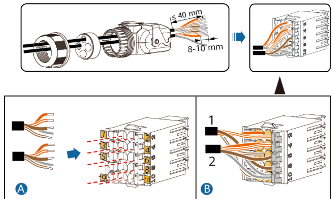
Figure 5-26 Installation des câbles
