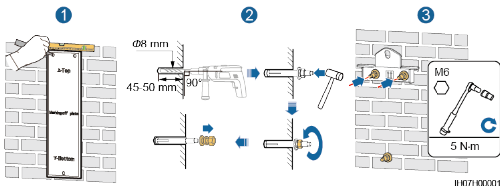
Figure 4-8 Installation des boulons extensibles
