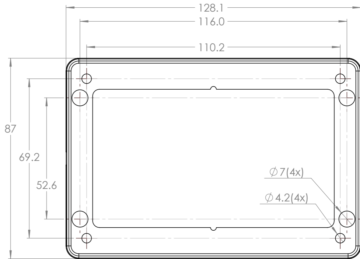
Frame dimensions
